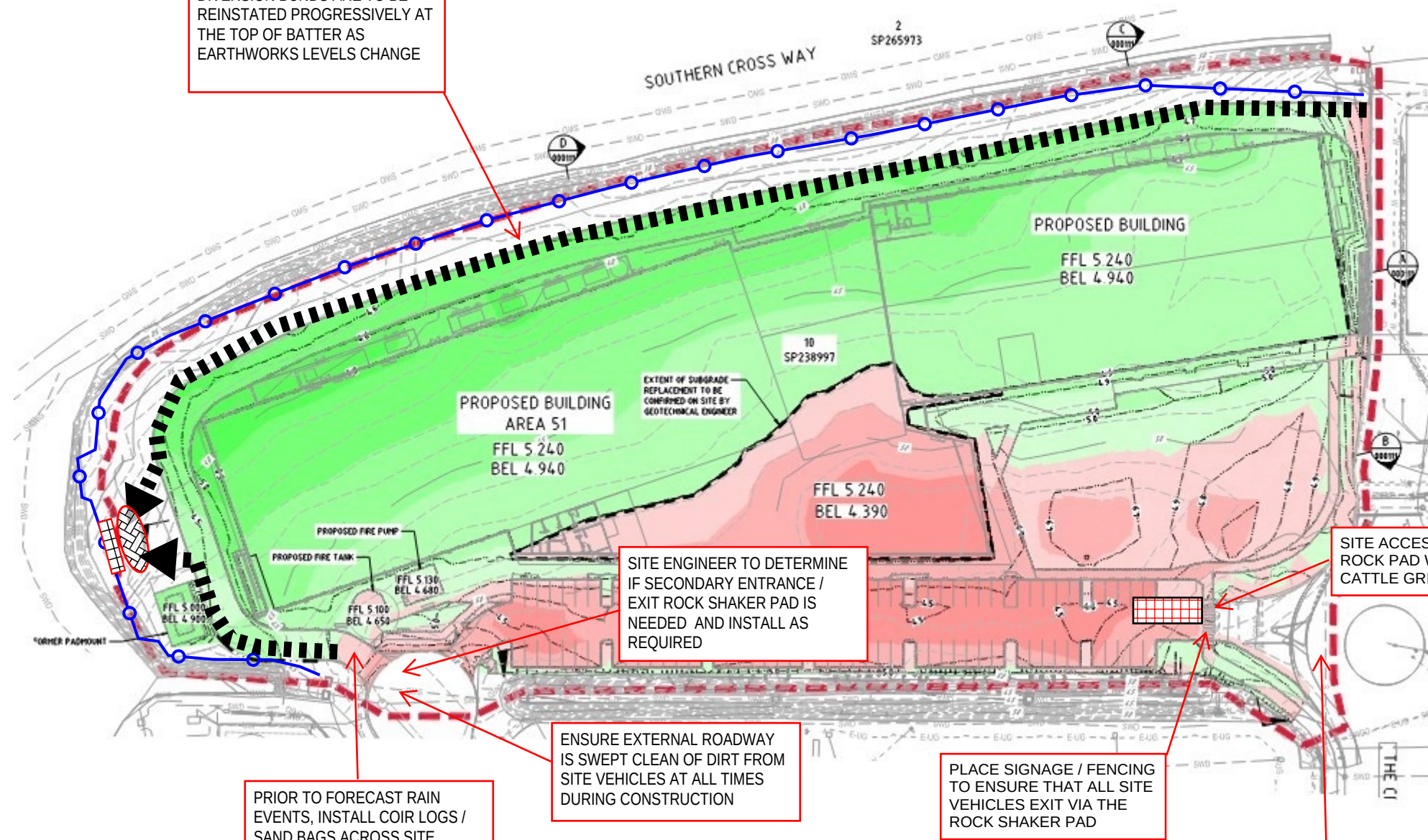
LAYOUT PLAN
